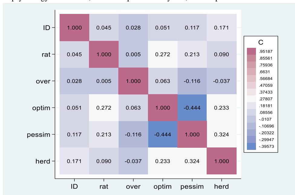
Figure 2: Correlation coefficient matrix between variables
